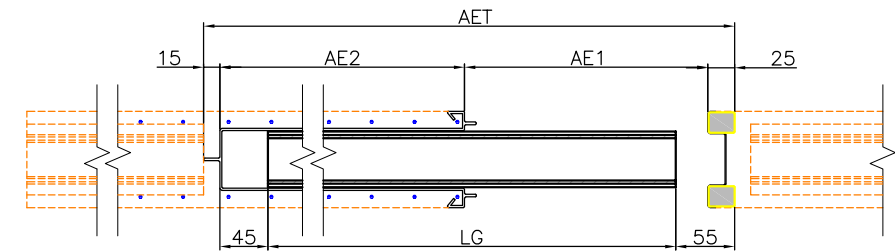
GUIDE SECTION SCALE, 1:5
